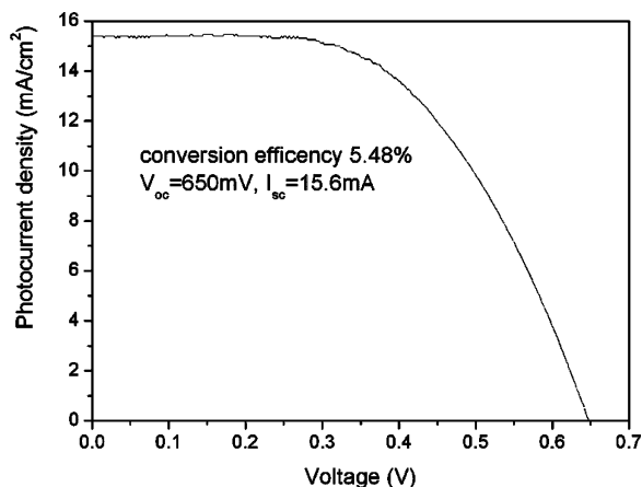
Figure 13. I – V curve of DSSC assembled with \text{LiI}(\text{HPN})_4/15 wt % \text{SiO}_2 (15 nm) under radiant power of 100 \text{ mW/cm}^2 (illumination area: 0.15 \text{ cm}^2 ).
