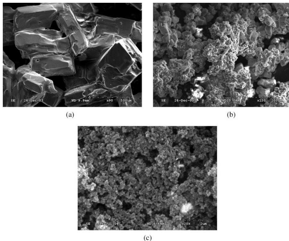
Figure 5. (a) SEM image of LiI/HPN (1:4) without SiO 2 , (b) SEM of LiI/HPN (1:4) containing 20 wt % μm-SiO 2 (0.3–2 μm), and (c) SEM of LiI(HPN) 4 containing 15 wt % nano-SiO 2 (15 nm).
